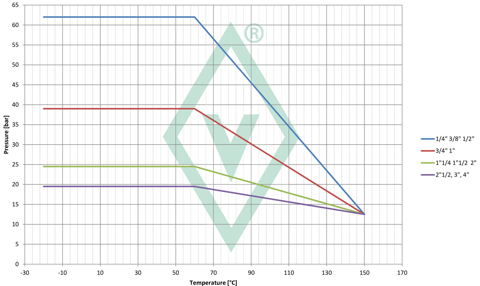
Pressure/Temperature Chart
